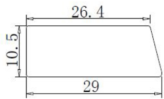
Unilateral cross-section 10:1
