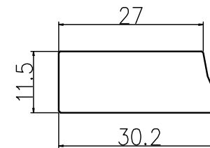
Unilateral cross-section 10:1
